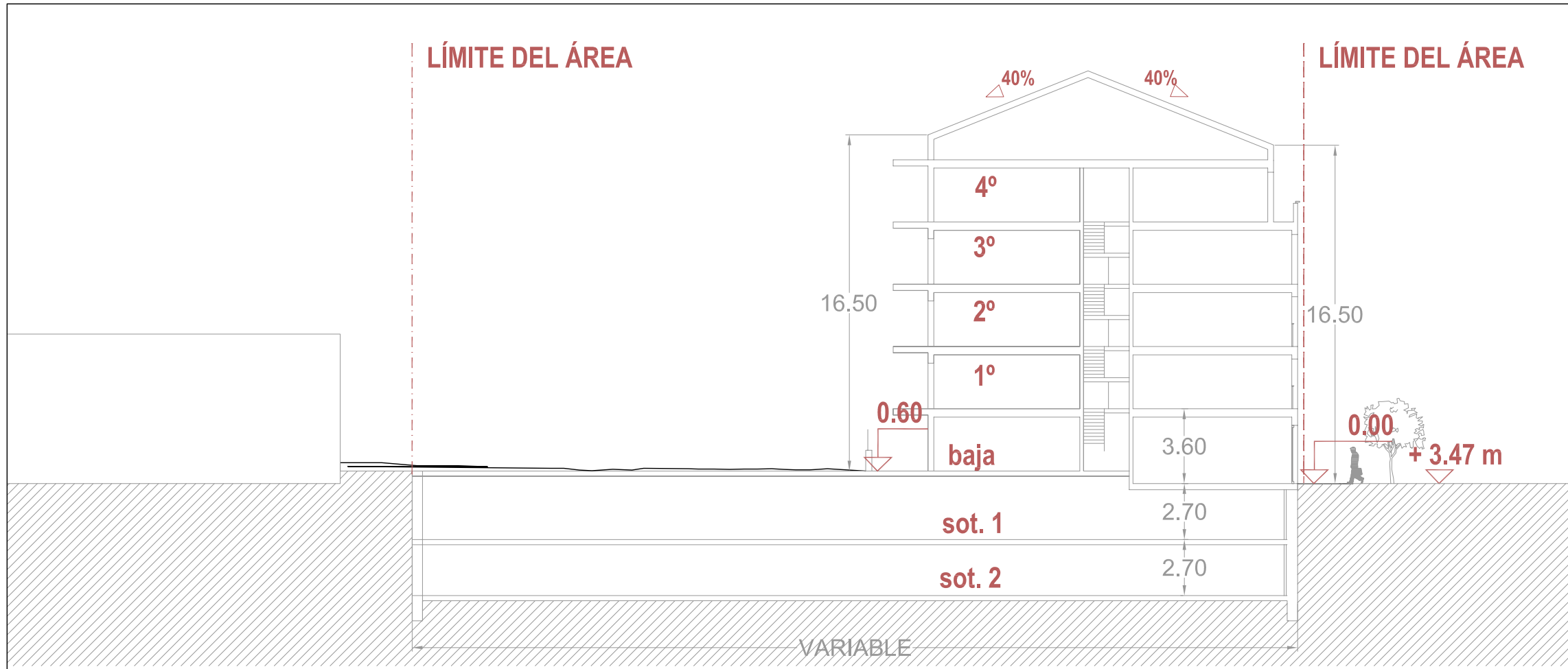
SECCION T1-T1'
