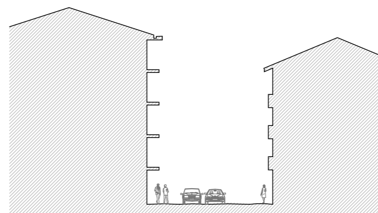
C/ SANTA ELENA SANTA ELENA KALEA E:1/300
