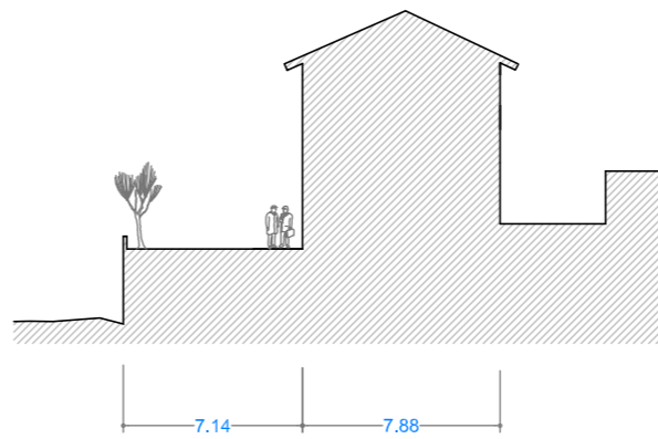
C/ ERMITA ERMITA KALEA E:1/300
